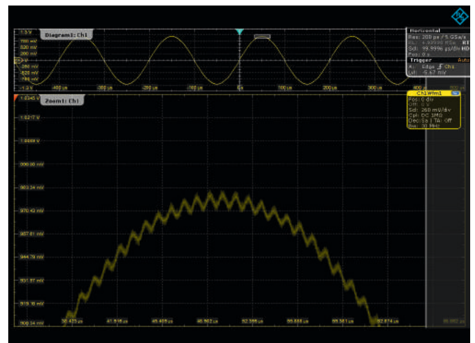
When the high definition mode is switched on, the zoom window shows that another very low-amplitude sine wave is superimposed on the signal.
