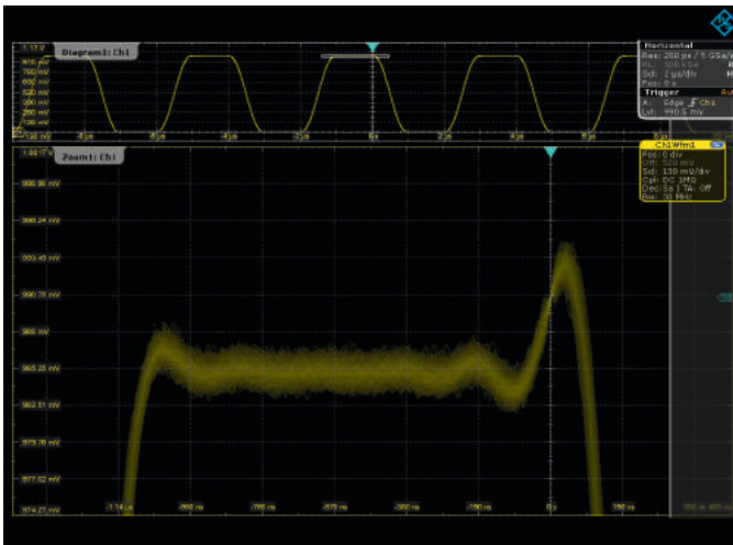
The high sensitivity of the Rohde & Schwarz digital trigger makes it possible to trigger on signal overshoots of less than 9 mV, as can be seen in this example. At a vertical scale of 130 mV/div, this corresponds to only a fraction of one display division.
