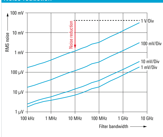
Noise of the R&S®RTO1044 oscilloscope (4 GHz model) as a function of the set filter bandwidth of the R&S®RTO-K17 high definition option; a reduction in noise leads to an increase in the signal-to-noise ratio, which improves the vertical resolution.
