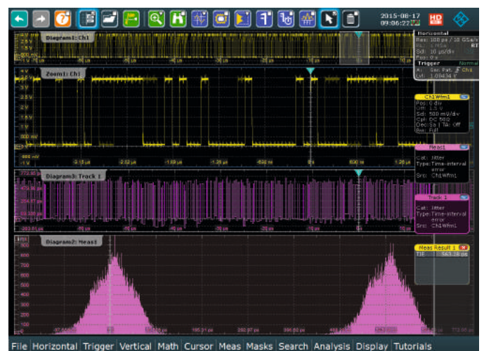
Measurement of the time interval error (TIE) of the embedded clock for different bit sequences (010000X10000001). The lower histogram shows that the TIE differs based on the bit sequence.
